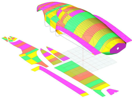
Cozy MkIV Canopy/Nose/Engine Cover, 3D model
