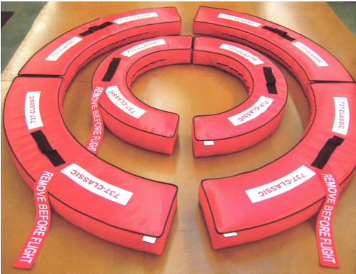
Boeing 737 Engine Intake Plug, Folding Type Boeing 737, Bypass & Exhaust Plugs, Folding Donut Ring Type, 300-500 Models
